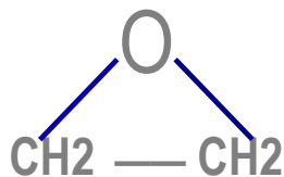
Chemical structure of EO
